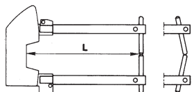
Art. 7501 L=125 mm Art. 7502 L=250 mm Art. 7503 L=350 mm Art. 7504 L=500 mm Art. 7521 \varnothing 10 ▲
